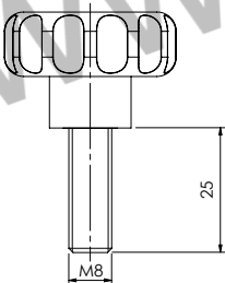
HANDKNOB CODE 62200012
