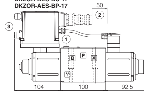
DKZOR-AES-BC-17 DKZOR-AES-BP-17
