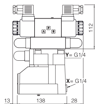
AGAM-20/32/**-LX
