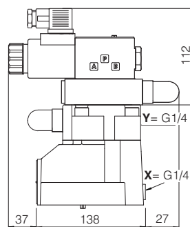
AGAM-20/22/**-EX
