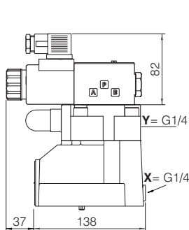
AGAM-20/10/**-EX AGAM-20/11/**-EX
