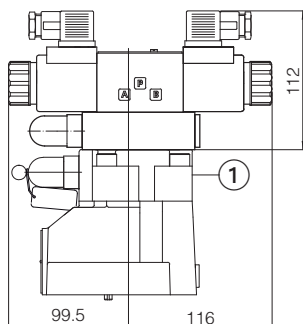
AGAM-20/20/**-EPX AGAM-20/21/**-EPX
