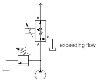
3 way connection
