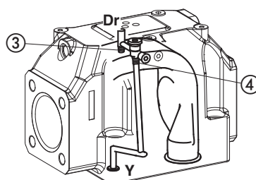
Drain channels
