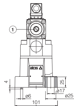
AGMZO-A-20
