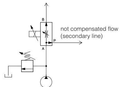
priority connection
