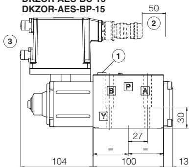
DKZOR-AES-BC-15 DKZOR-AES-BP-15
