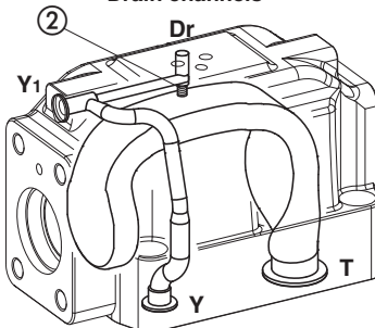
Drain channels
