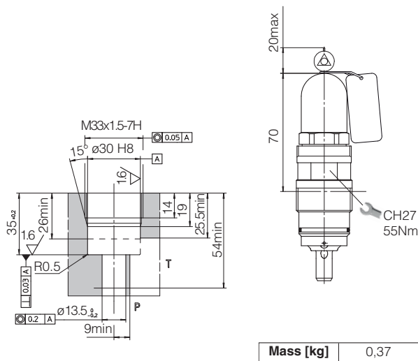
CART ARE-20
