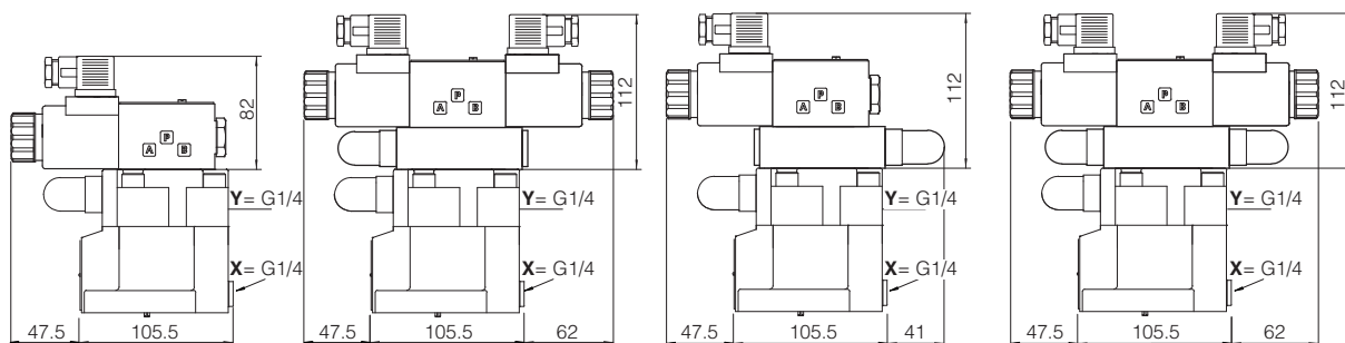
AGAM-10/10/**-EX AGAM-10/11/**-EX
