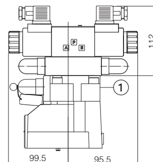
AGAM-20/32/**-EPX
