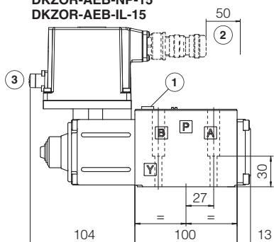
DKZOR-AEB-NP-15 DKZOR-AEB-IL-15
