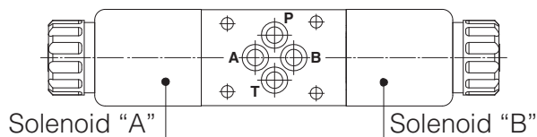
Fig. 2 Solenoid identification
