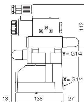
AGAM-20/22/**-LX
