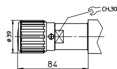
Adjustment device for option /VF and /VS
