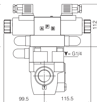
ARAM-20/32/**-EX
