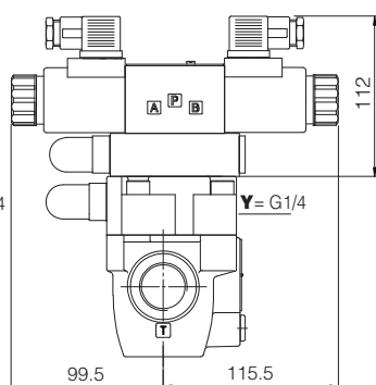
ARAM-20/20/**-EX ARAM-20/21/**-EX
