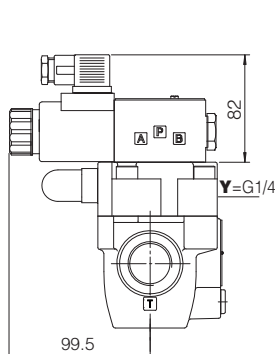
ARAM-20/10/**-EX ARAM-20/11/**-EX
