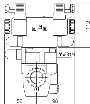
ARAM-20/32/**-LX
