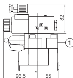
AGAM-10/10/**-EPX AGAM-10/11/**-EPX
