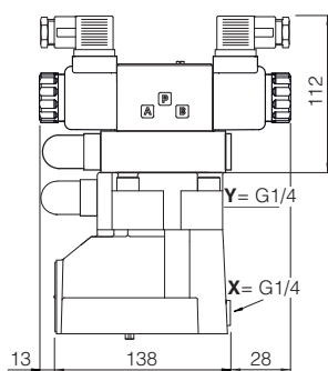
AGAM-20/20/**-LX AGAM-20/21/**-LX
