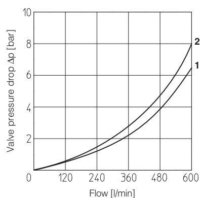
size 25
