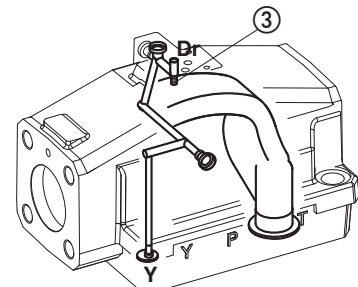
Drain channels
