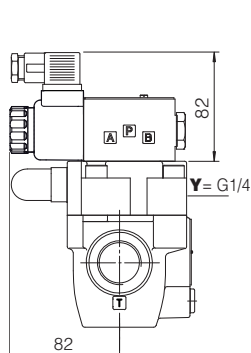
ARAM-20/10/**-LX ARAM-20/11/**-LX
