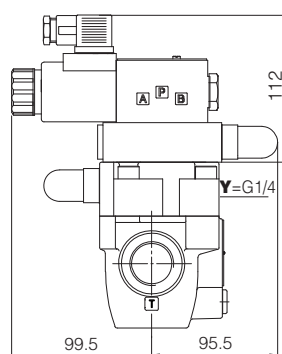
ARAM-20/22/**-EX
