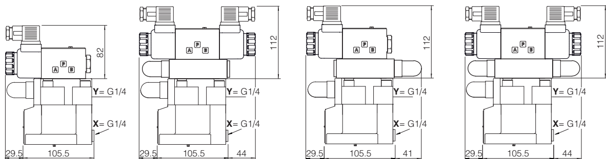
AGAM-10/10/**-LX AGAM-10/11/**-LX
