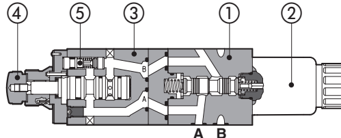
DHQ-013/*-EX*
