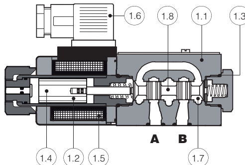
Fig. 1 Cross-section of direct operated solenoid valve
