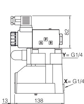
AGAM-20/10/**-LX AGAM-20/11/**-LX
