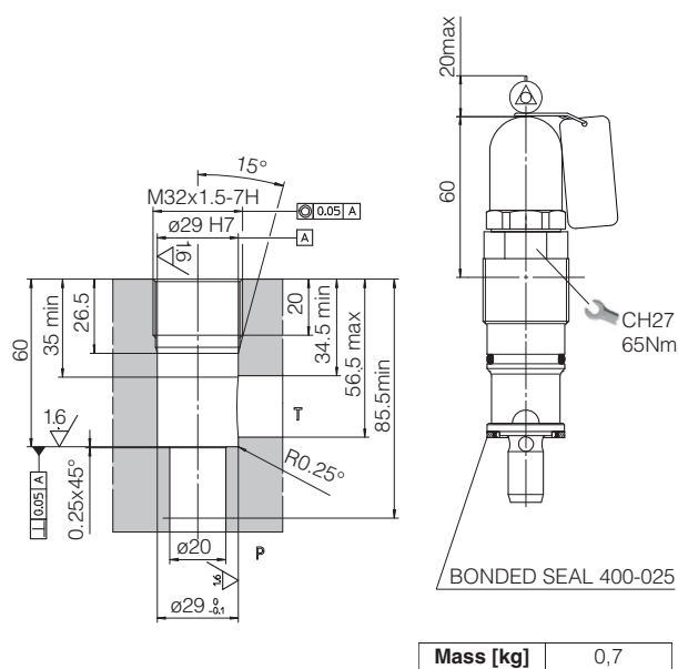
CART ARE-15
