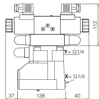
AGAM-20/32/**-EX
